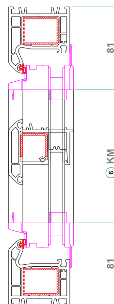
Section C-C
