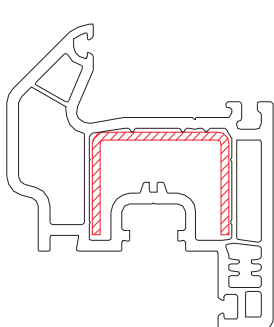
Sash S-507.02
