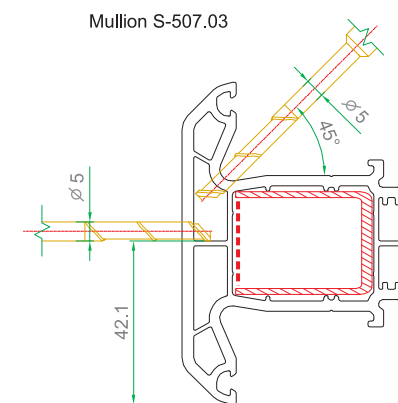
Mullion S-507.03
