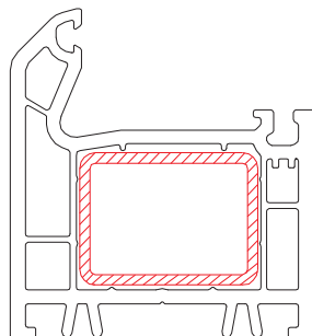
Frame S-507.01
