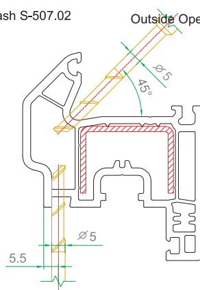
Sash S-507.02
