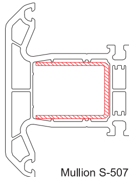
Mullion S-507.03
